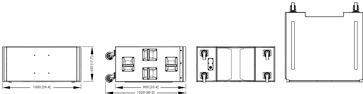
KSL-GSUB cabinet dimensions in mm [inch]
